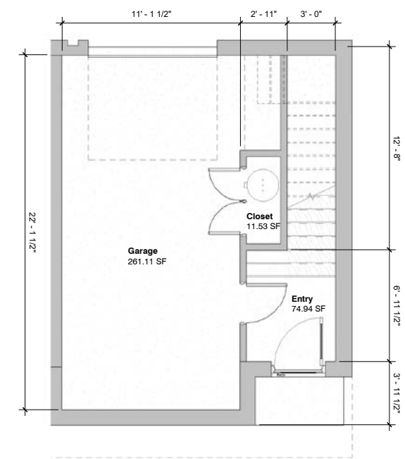
Level 01
