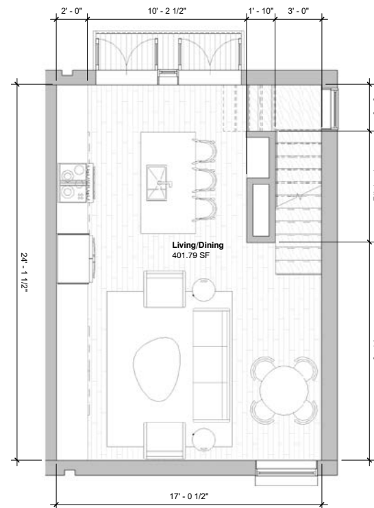
Level 02
