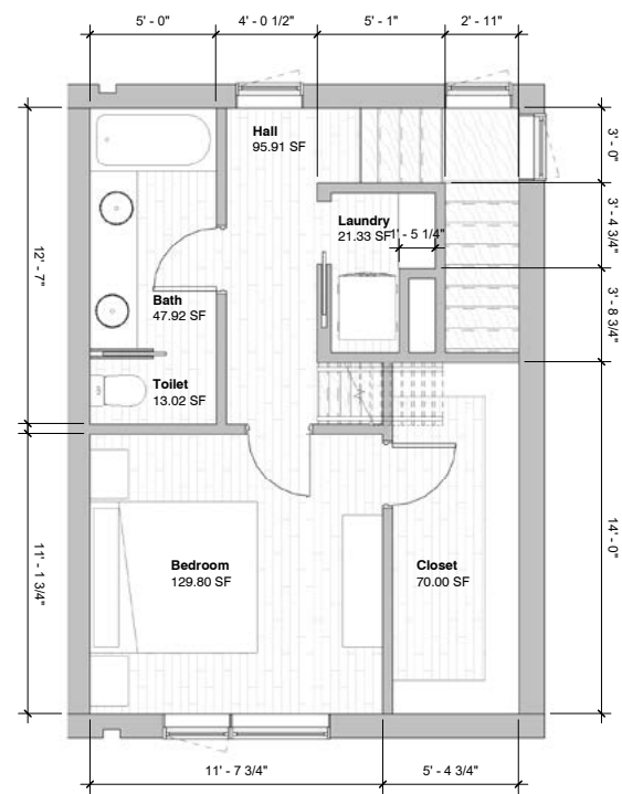
Level 03
