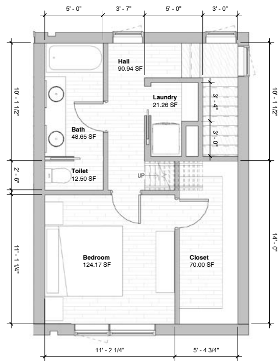
Level 03
