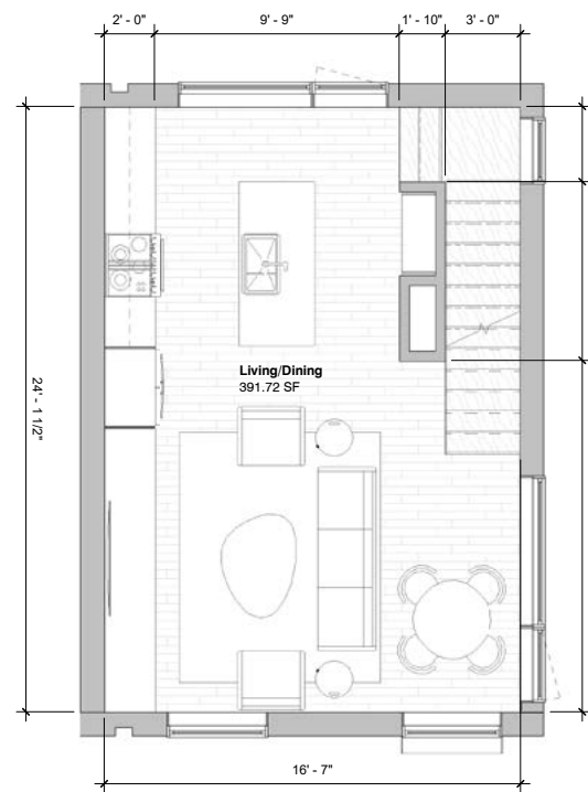
Level 02
