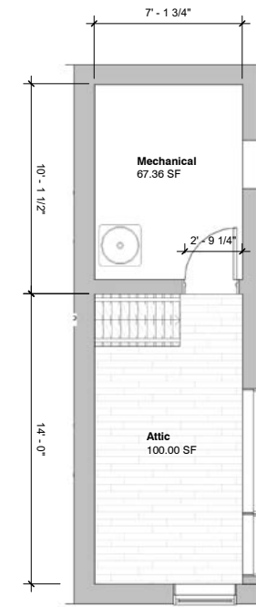
Attic/Mechanical
